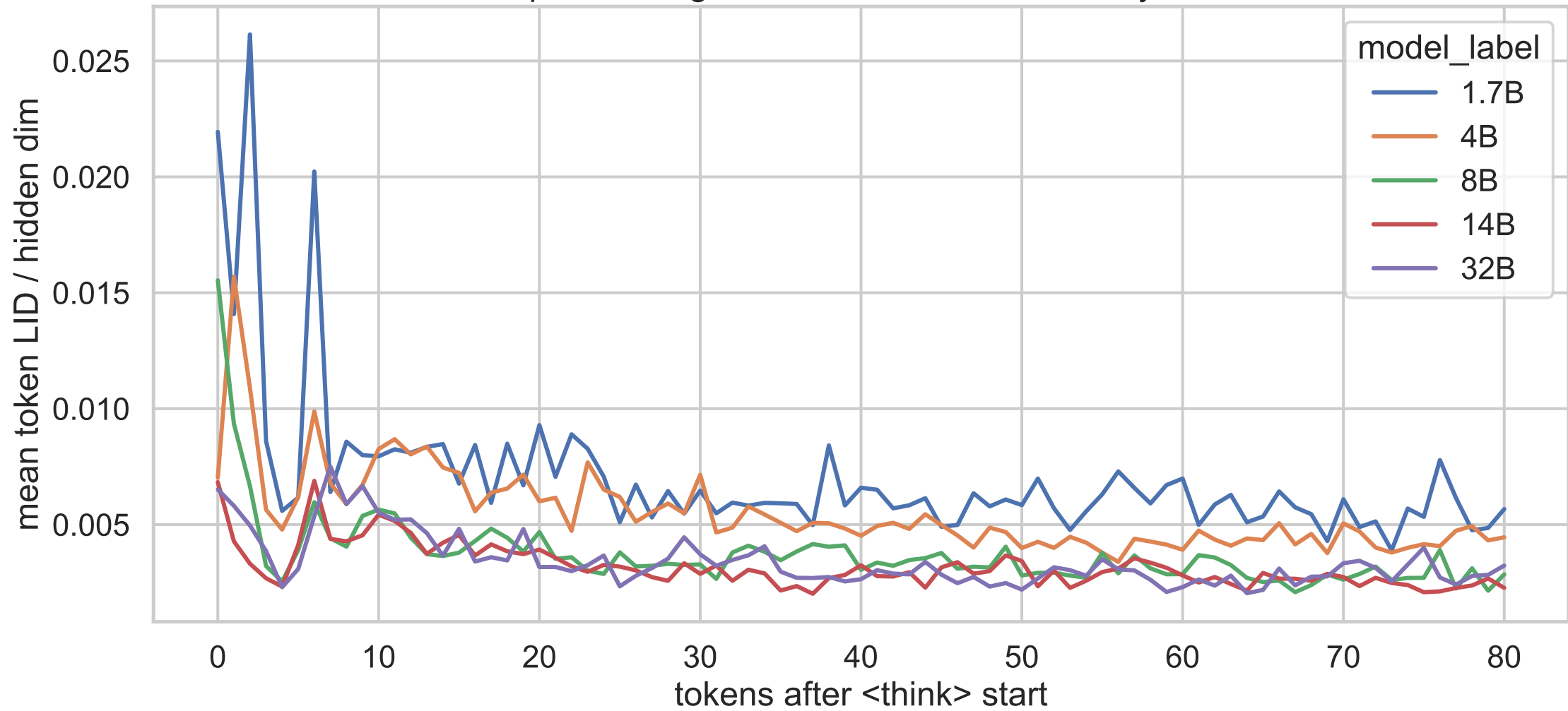
Exp C thinking-start anchored mean LID, layer 13
