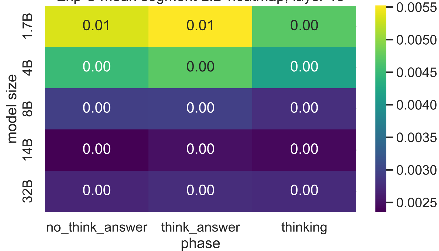
Exp C mean segment LID heatmap, layer 13
