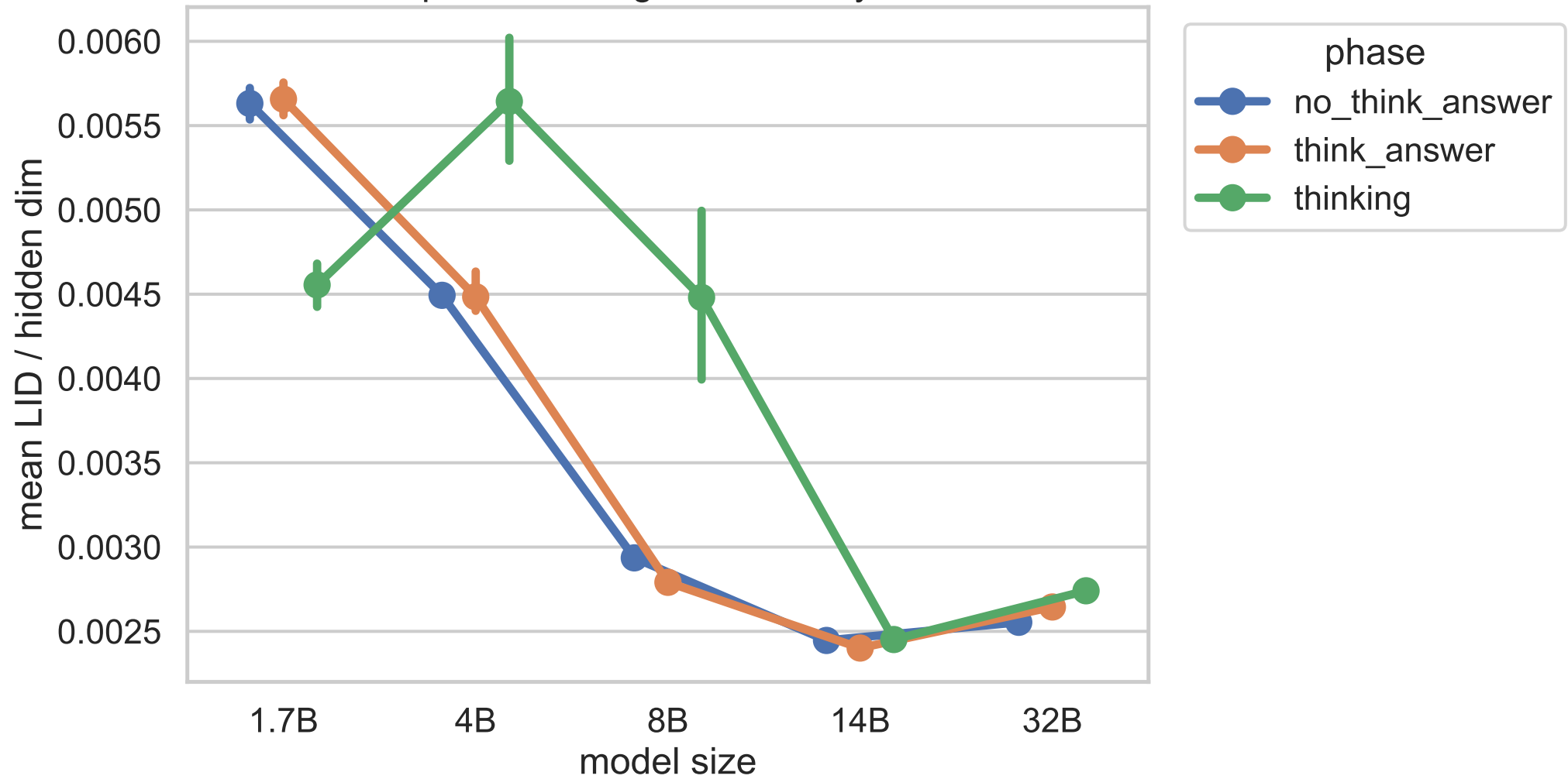
Exp C mean segment LID, layer 20
