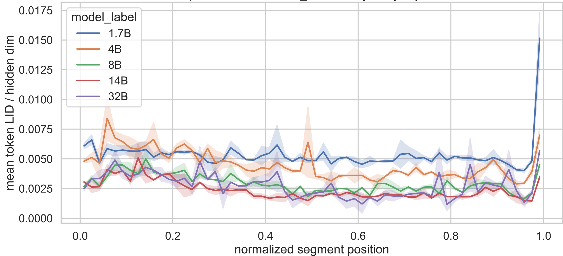
Exp C normalized think_answer trajectory, layer 13
