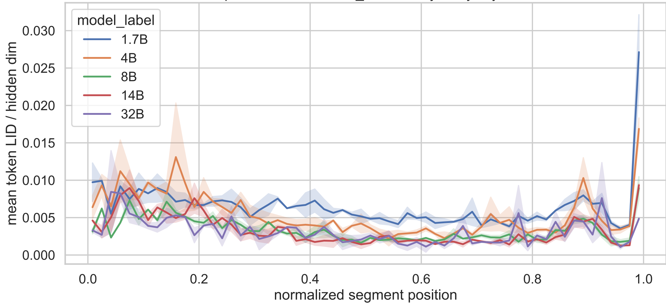
Exp C normalized think_answer trajectory, layer 6
