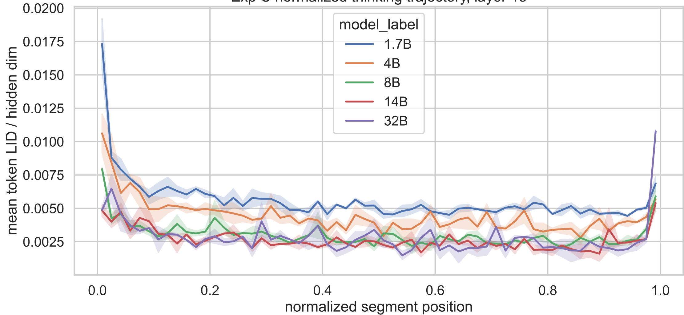
Exp C normalized thinking trajectory, layer 13
