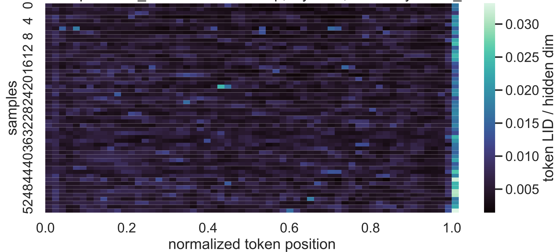
1.7B Exp C think_answer LID heatmap, layer 13, sorted by mean_lid
