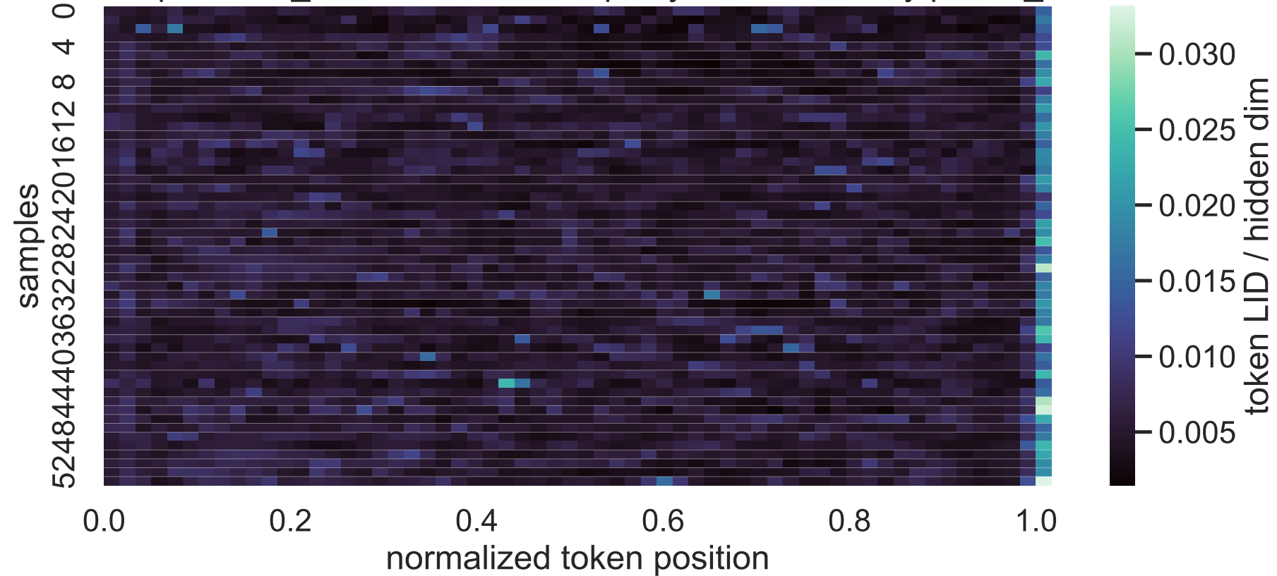
1.7B Exp C think_answer LID heatmap, layer 13, sorted by paired_delta
