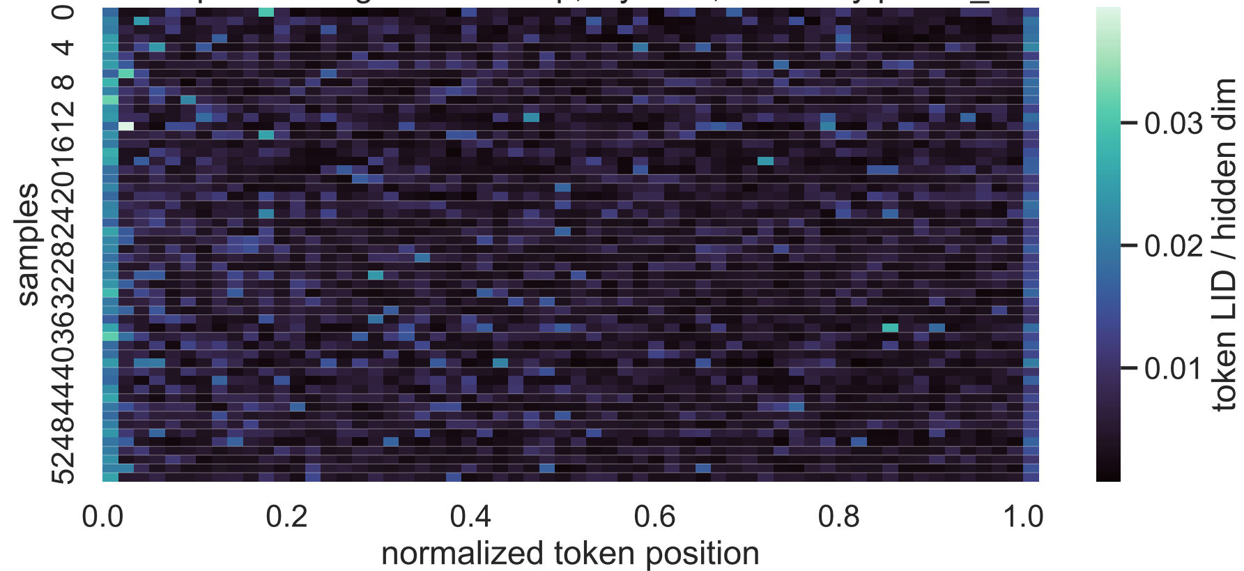
1.7B Exp C thinking LID heatmap, layer 13, sorted by paired_delta
