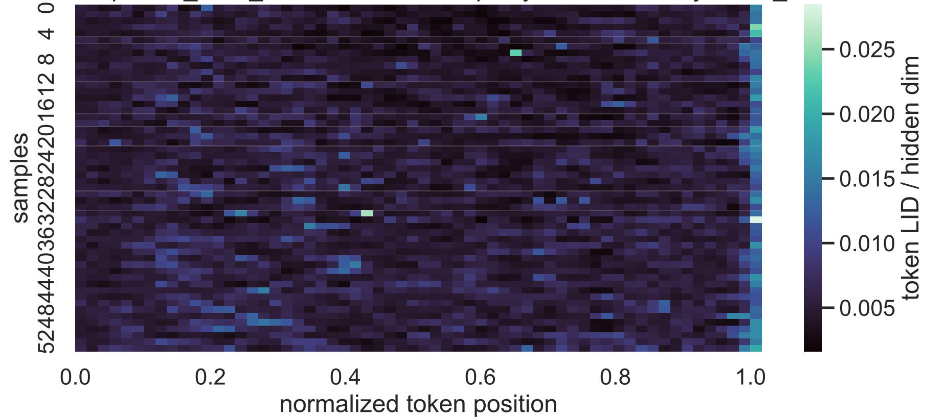
1.7B Exp C no_think_answer LID heatmap, layer 20, sorted by mean_lid
