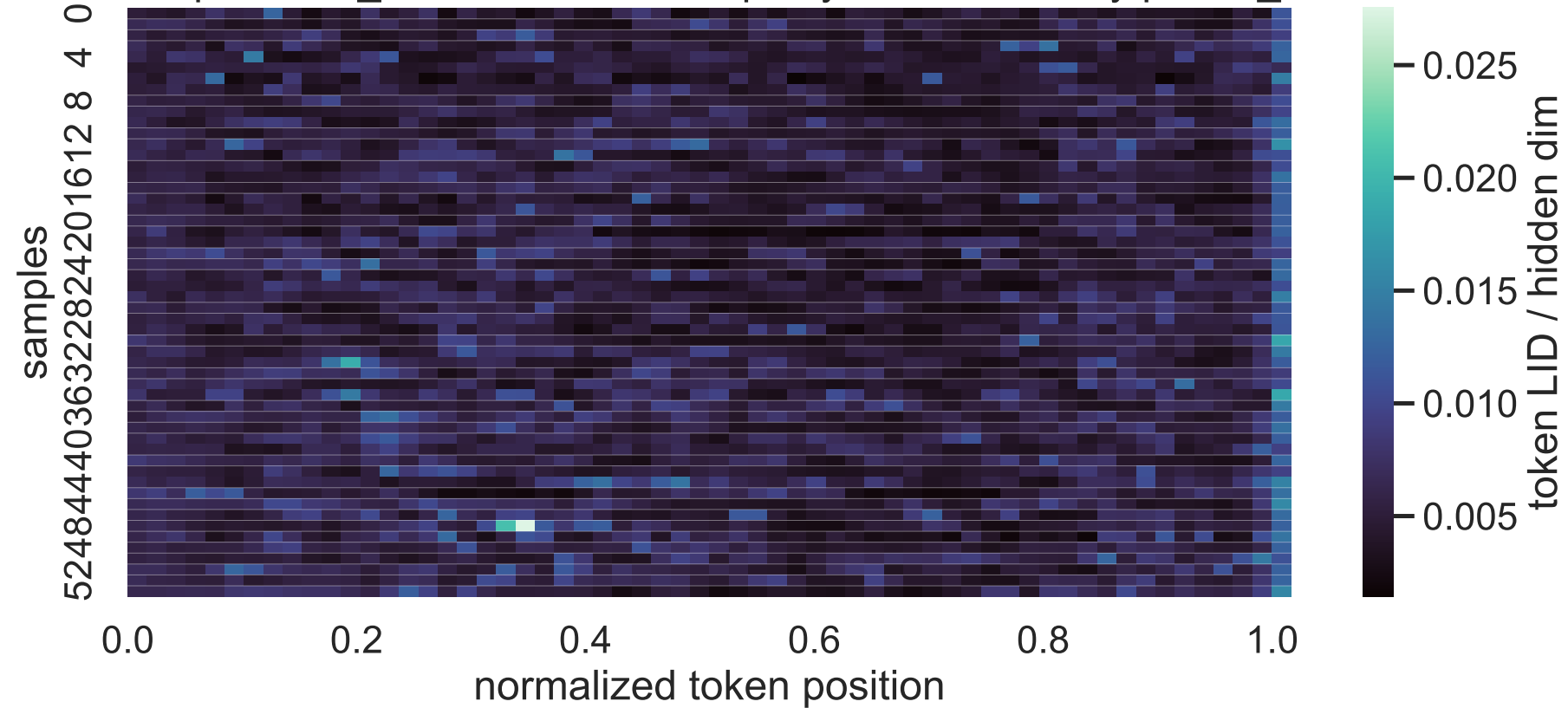
1.7B Exp C think_answer LID heatmap, layer 20, sorted by paired_delta
