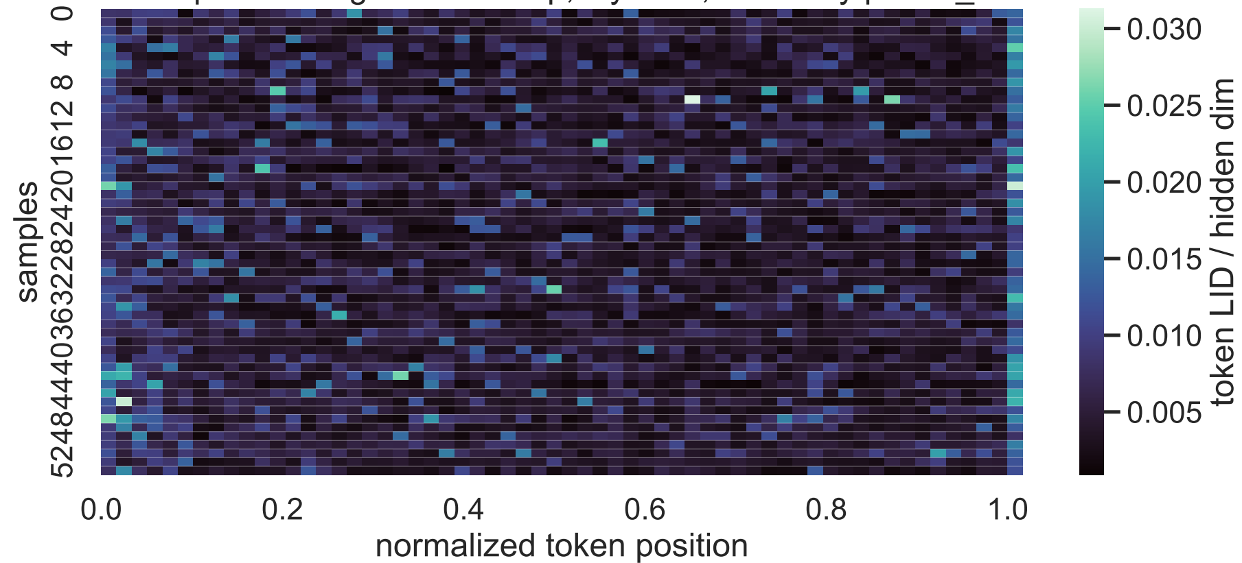
1.7B Exp C thinking LID heatmap, layer 20, sorted by paired_delta
