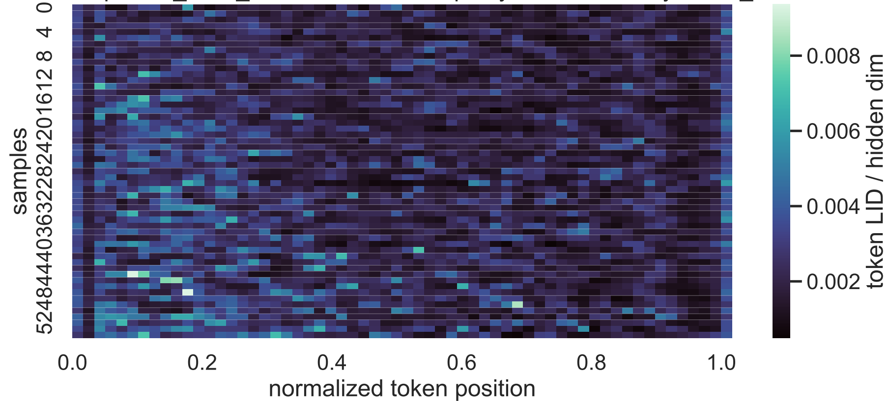
14B Exp C no_think_answer LID heatmap, layer 13, sorted by mean_lid
