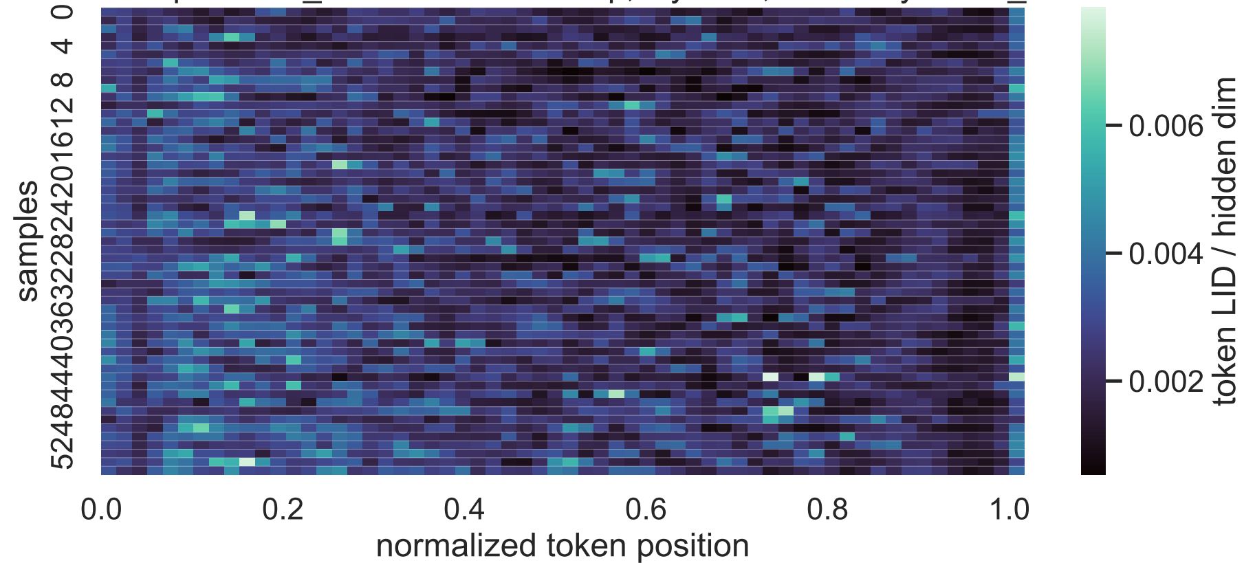
14B Exp C think_answer LID heatmap, layer 20, sorted by mean_lid
