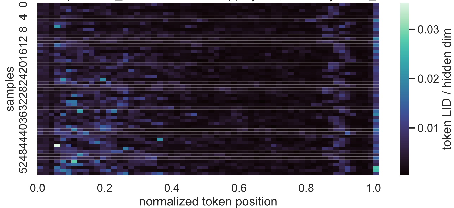
14B Exp C think_answer LID heatmap, layer 6, sorted by mean_lid
