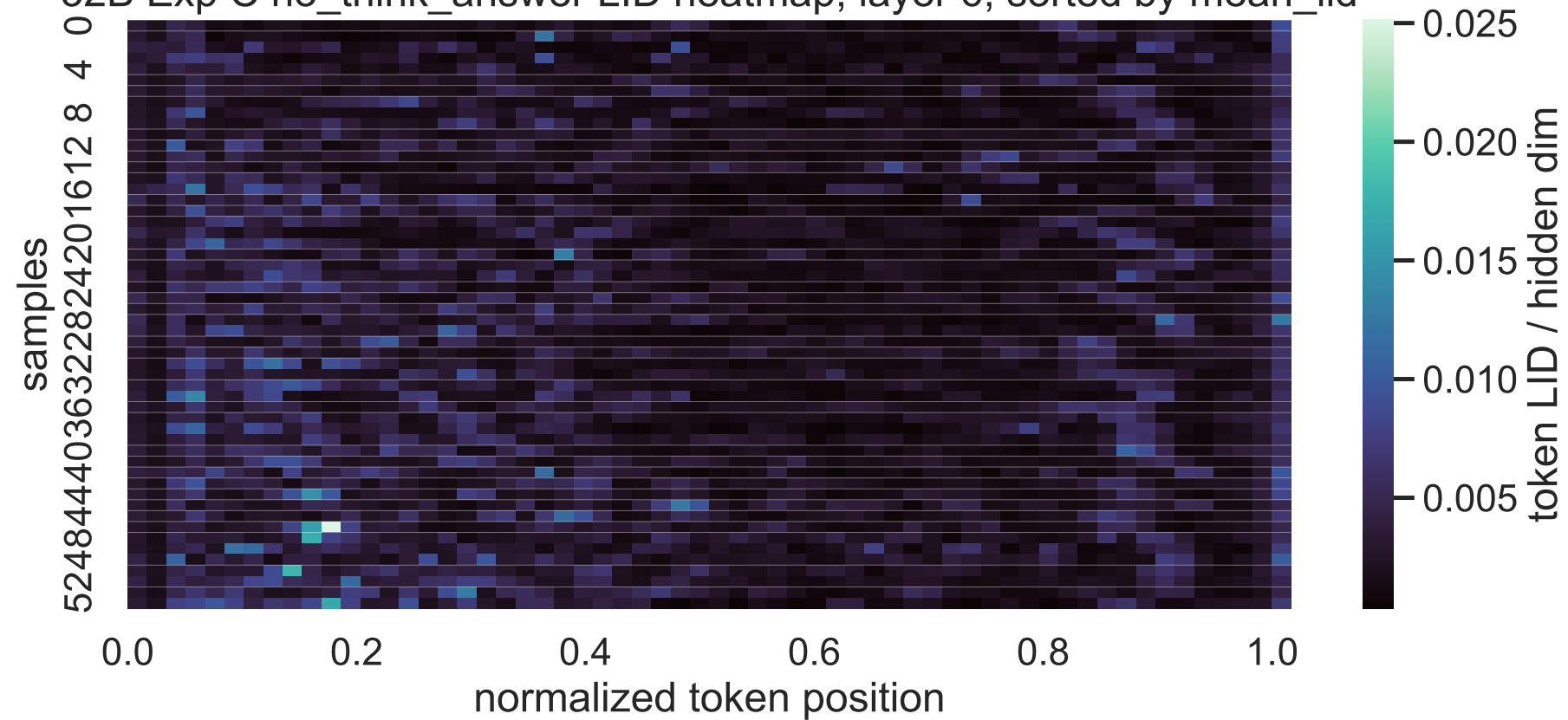
32B Exp C no_think_answer LID heatmap, layer 6, sorted by mean_lid
