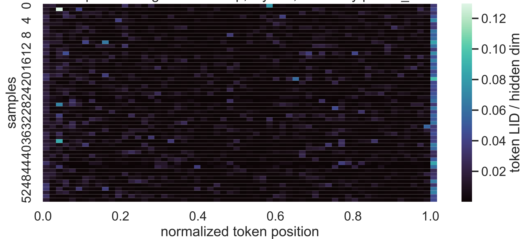
32B Exp C thinking LID heatmap, layer 6, sorted by paired_delta
