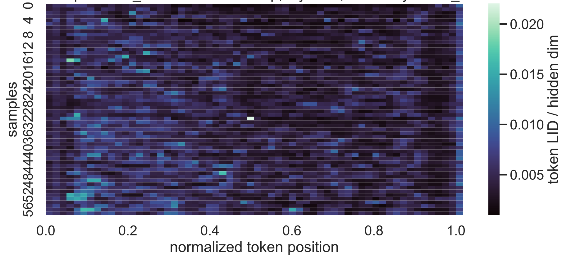
4B Exp C think_answer LID heatmap, layer 13, sorted by mean_lid
