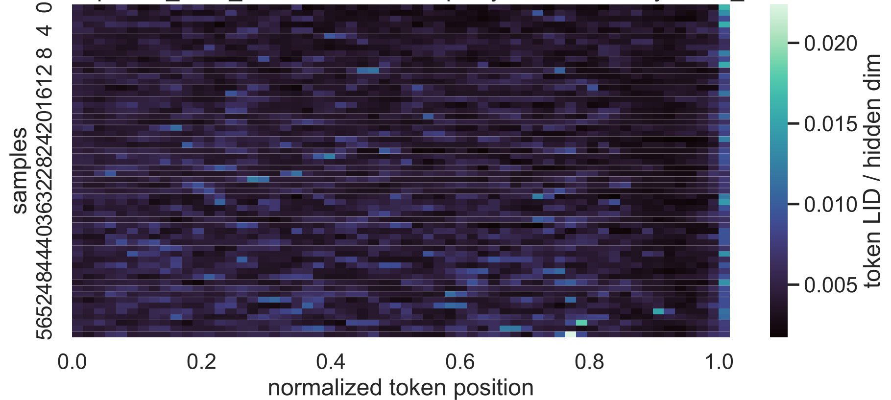
4B Exp C no_think_answer LID heatmap, layer 20, sorted by mean_lid
