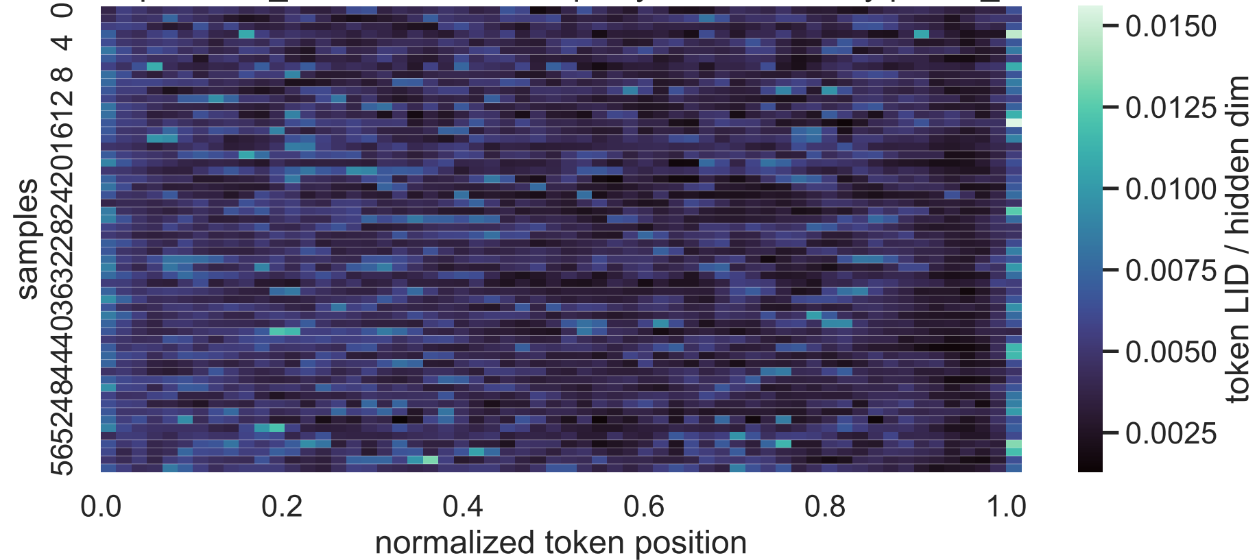
4B Exp C think_answer LID heatmap, layer 20, sorted by paired_delta
