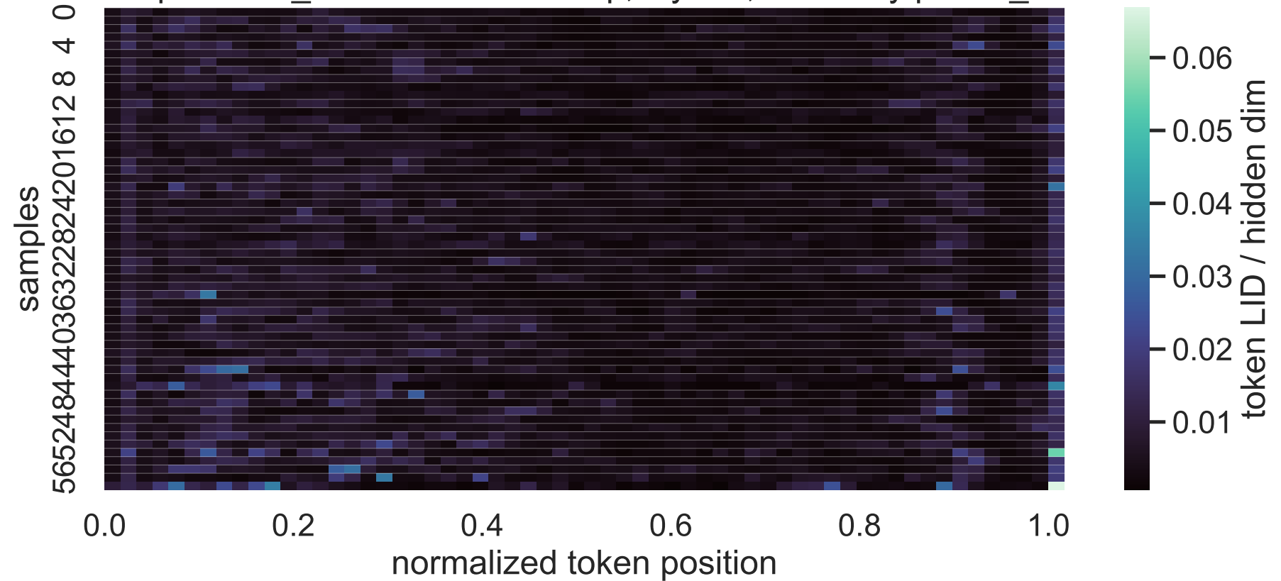
4B Exp C think_answer LID heatmap, layer 6, sorted by paired_delta
