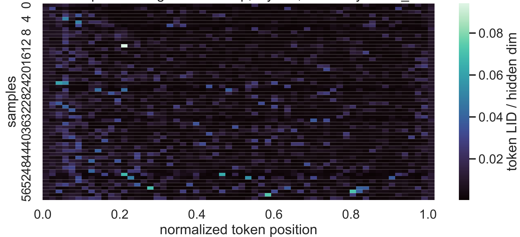
4B Exp C thinking LID heatmap, layer 6, sorted by mean_lid
