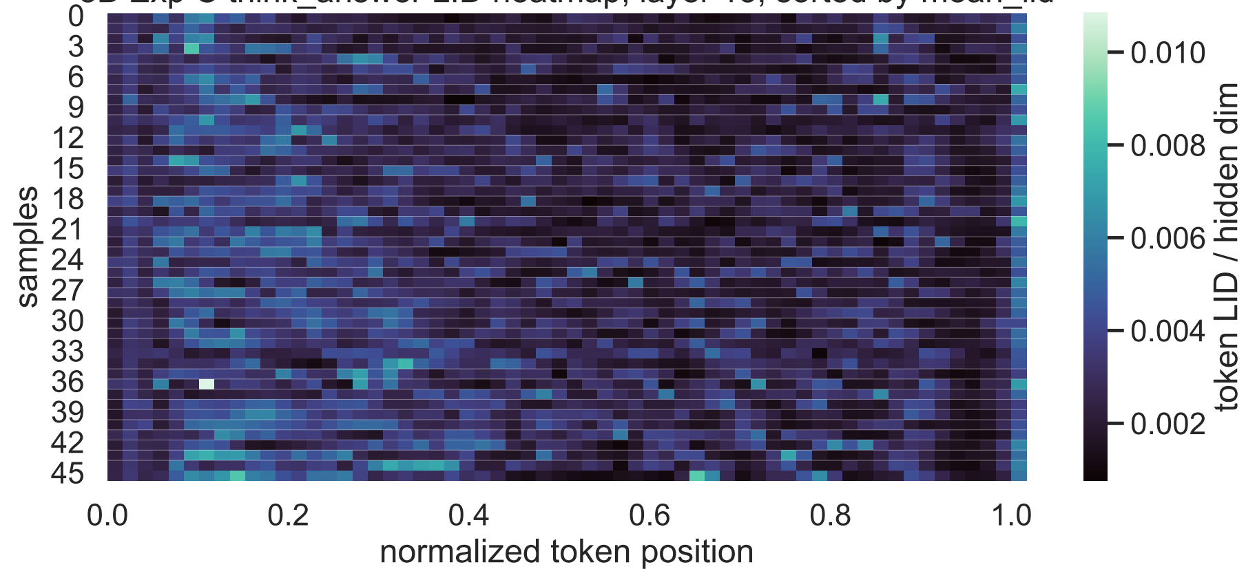
8B Exp C think_answer LID heatmap, layer 13, sorted by mean_lid
