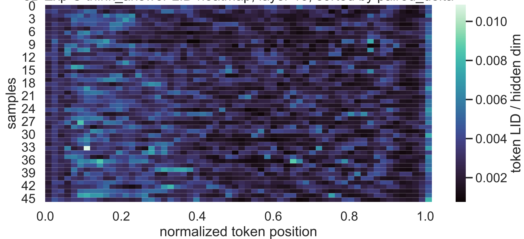
8B Exp C think_answer LID heatmap, layer 13, sorted by paired_delta
