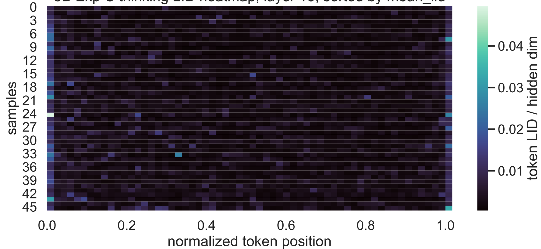
8B Exp C thinking LID heatmap, layer 13, sorted by mean_lid
