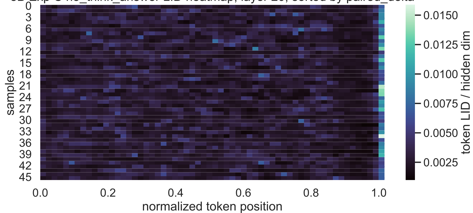
8B Exp C no_think_answer LID heatmap, layer 20, sorted by paired_delta
