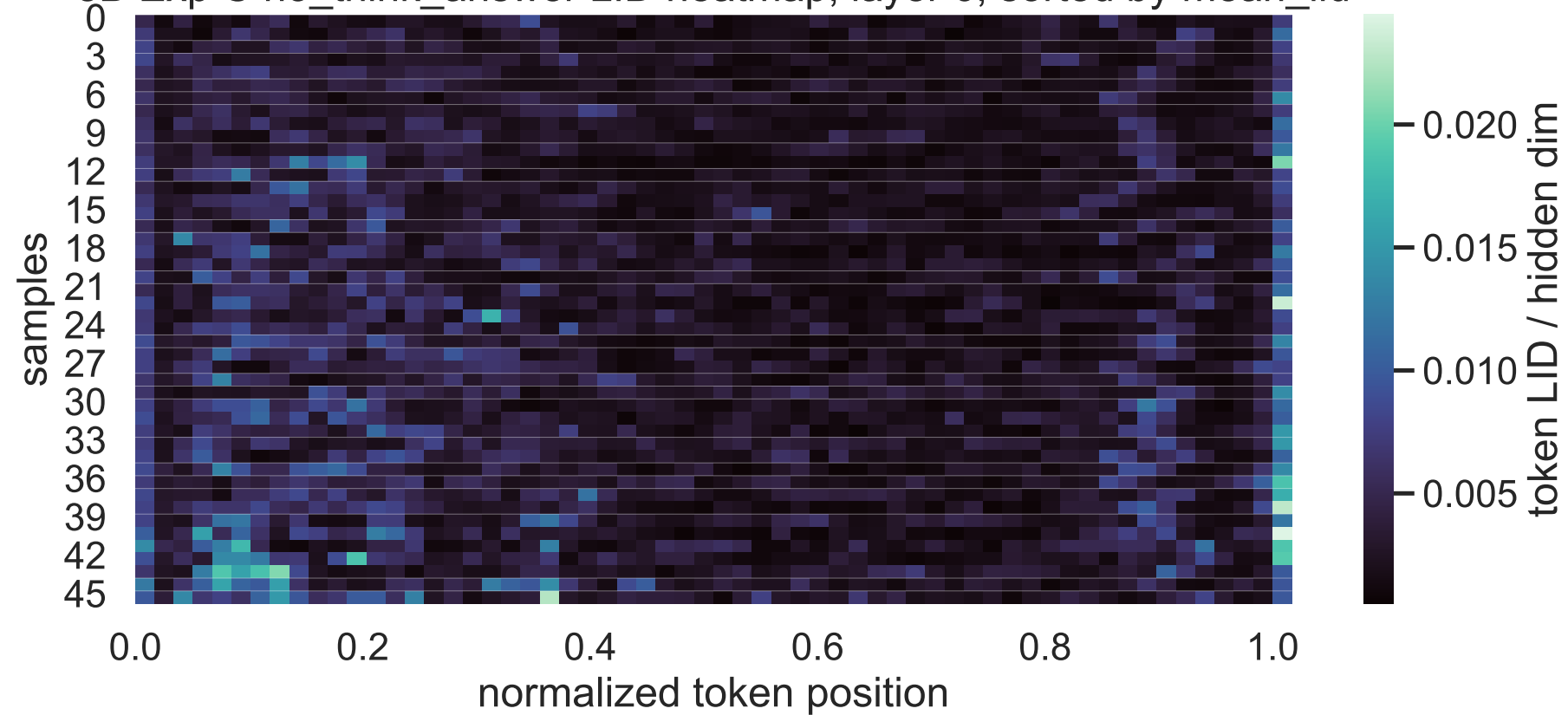
8B Exp C no_think_answer LID heatmap, layer 6, sorted by mean_lid
