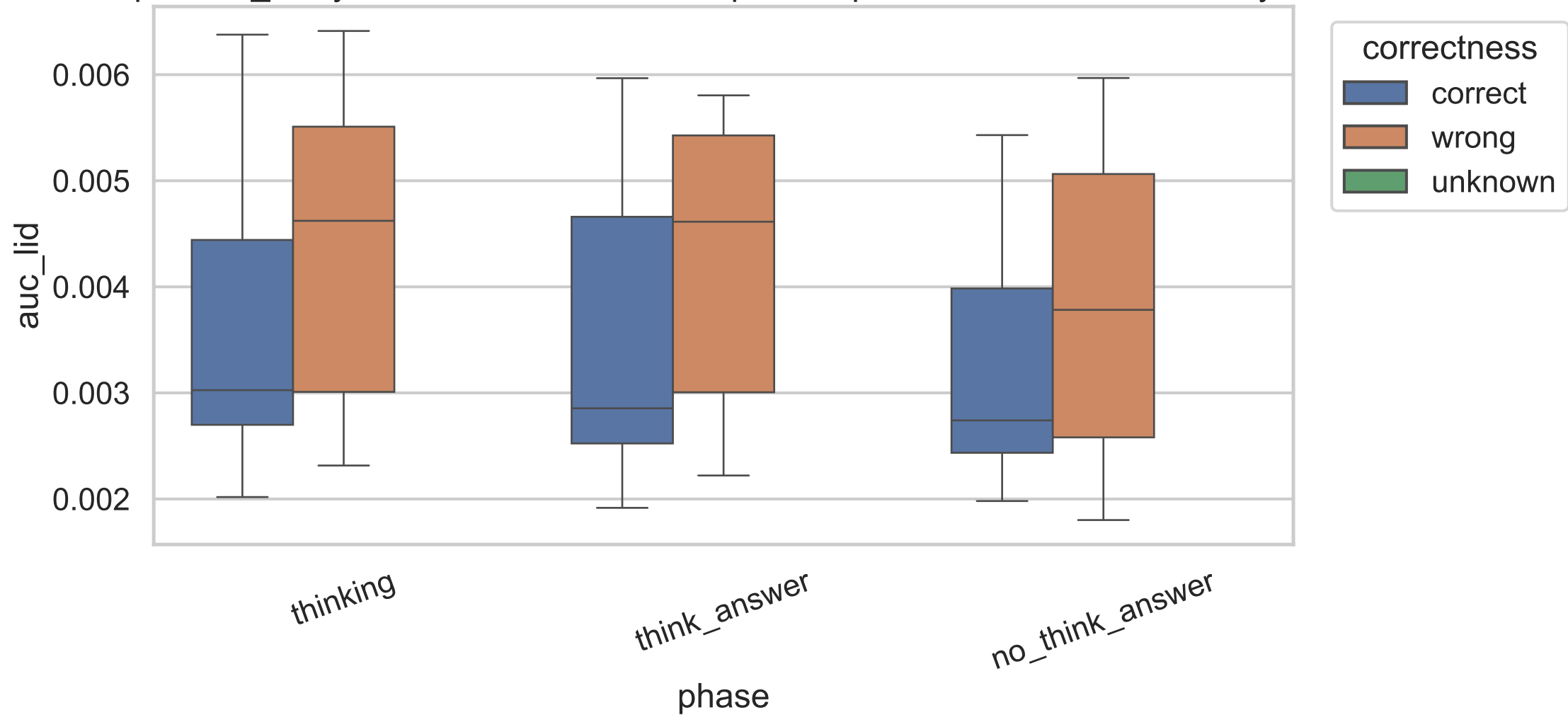
Exp C auc_lid by correctness, common-kept examples across model sizes, layer 13
