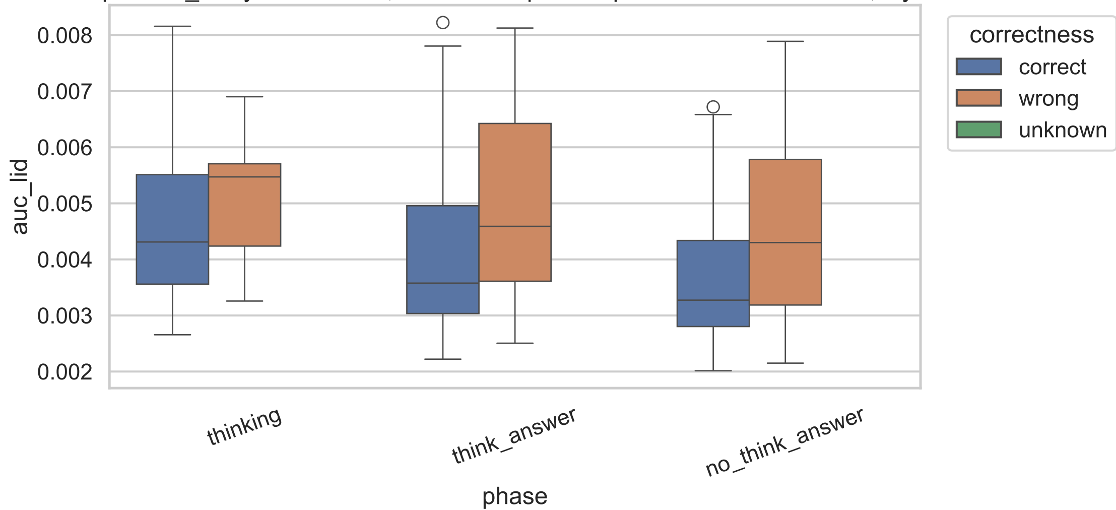
Exp C auc_lid by correctness, common-kept examples across model sizes, layer 6
