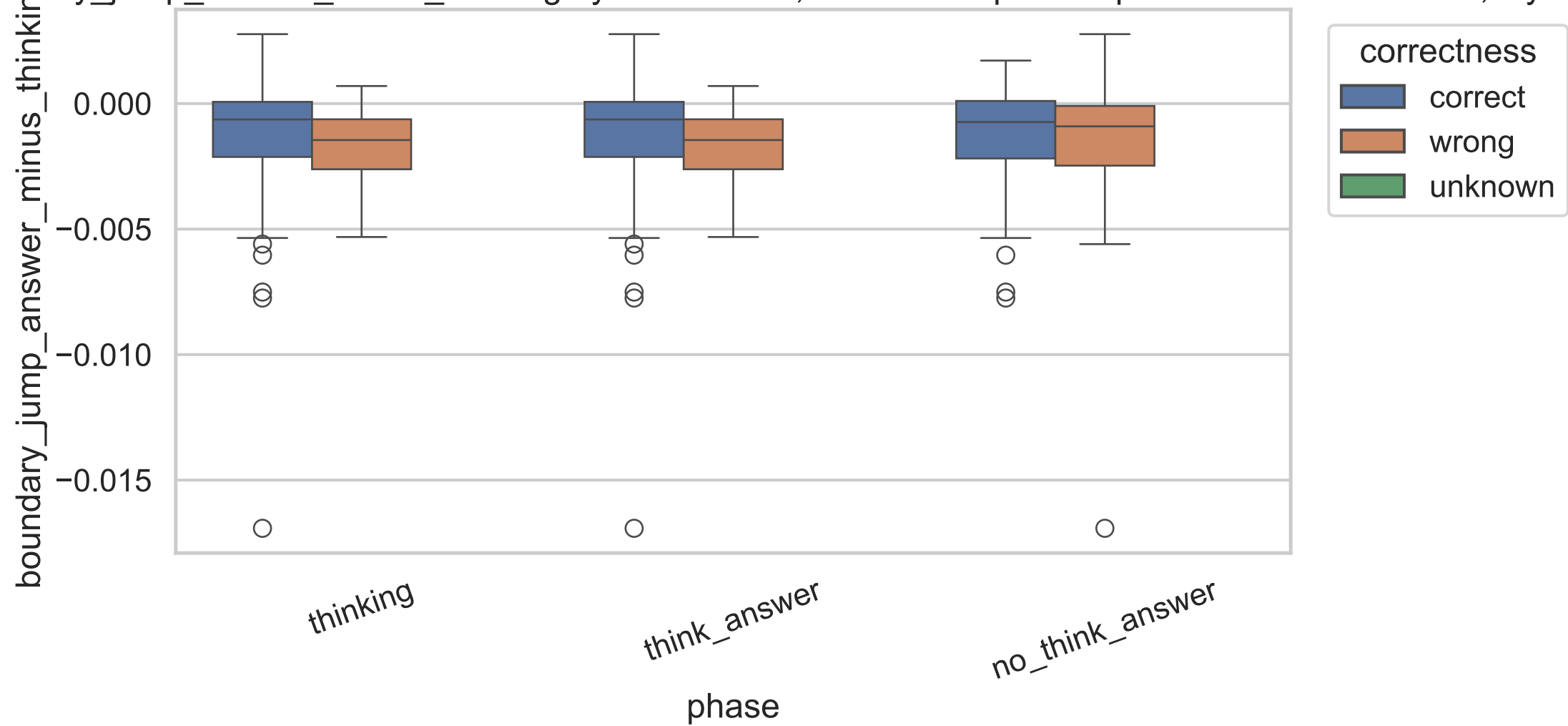
Exp C boundary_jump_answer_minus_thinking by correctness, common-kept examples across model sizes, layer 20
