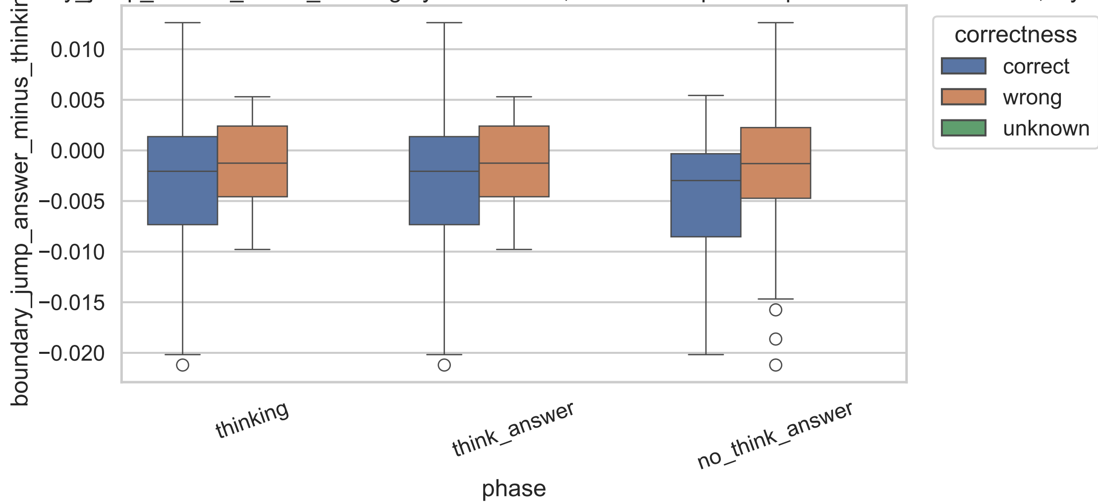
Exp C boundary_jump_answer_minus_thinking by correctness, common-kept examples across model sizes, layer 6
