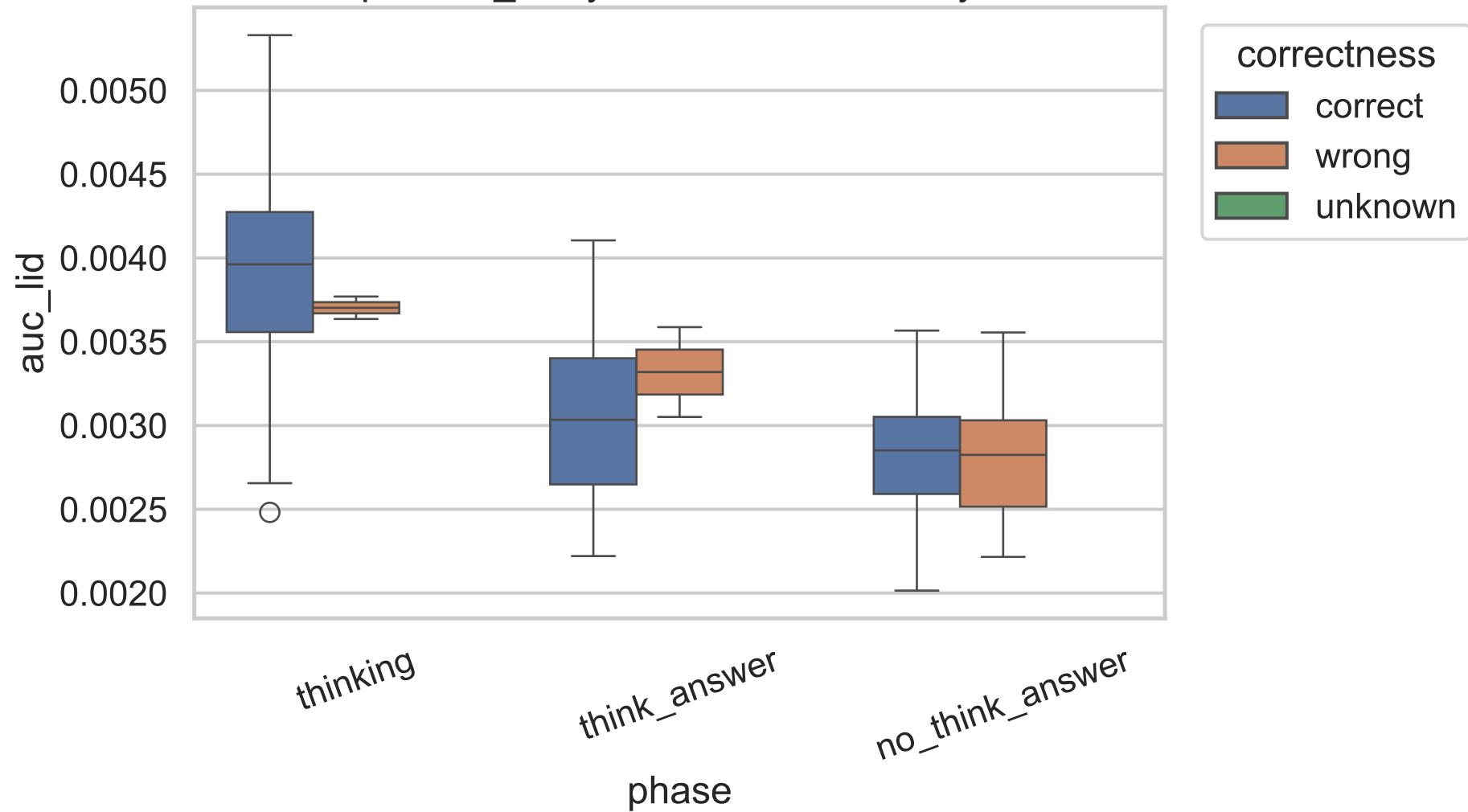
Exp C auc_lid by correctness, 32B, layer 6
