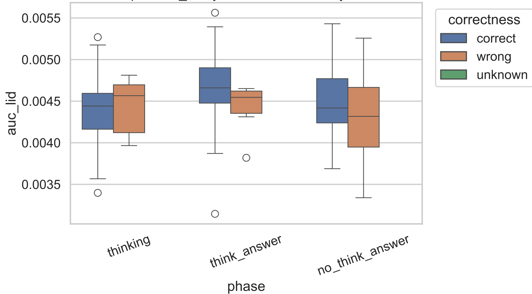
Exp C auc_lid by correctness, 4B, layer 13
