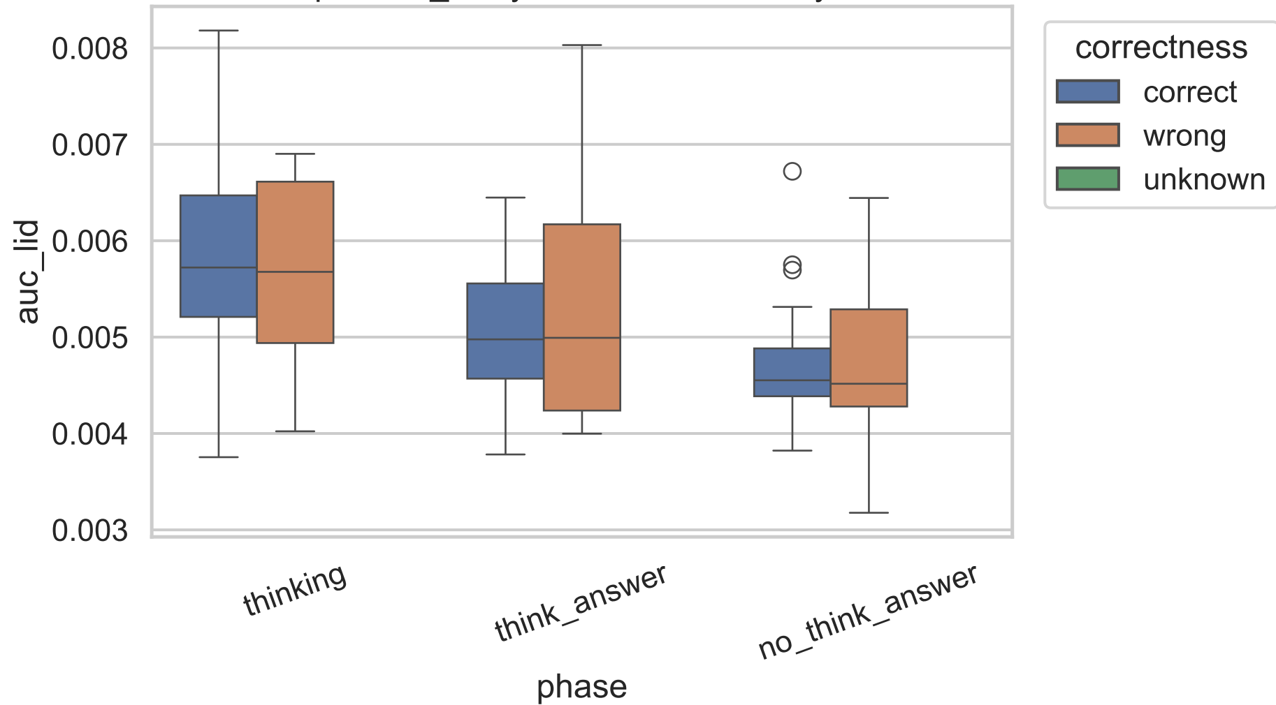
Exp C auc_lid by correctness, 4B, layer 6
