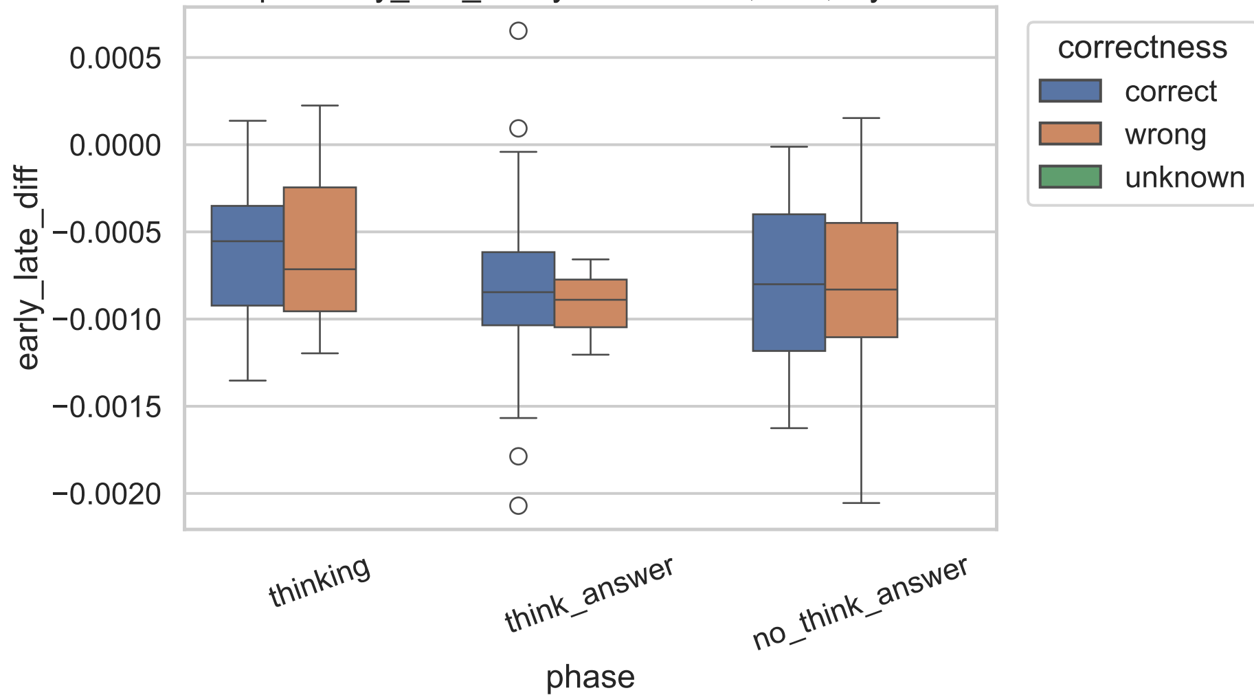
Exp C early_late_diff by correctness, 14B, layer 20
