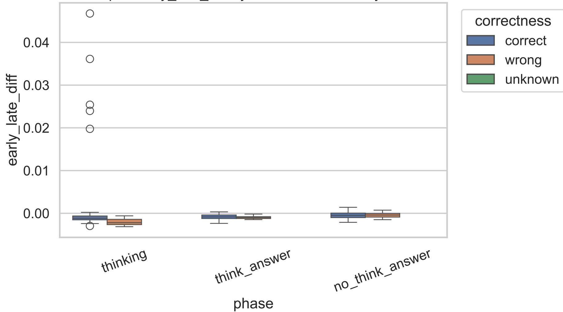
Exp C early_late_diff by correctness, 4B, layer 20
