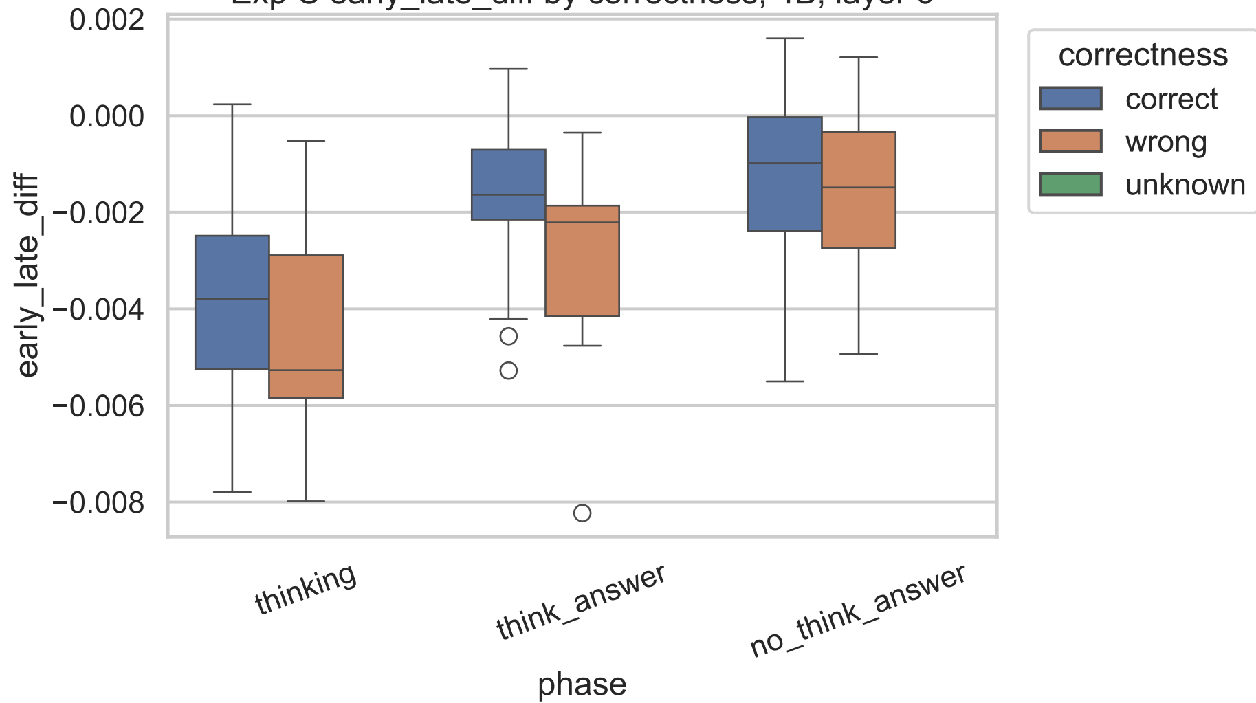
Exp C early_late_diff by correctness, 4B, layer 6
