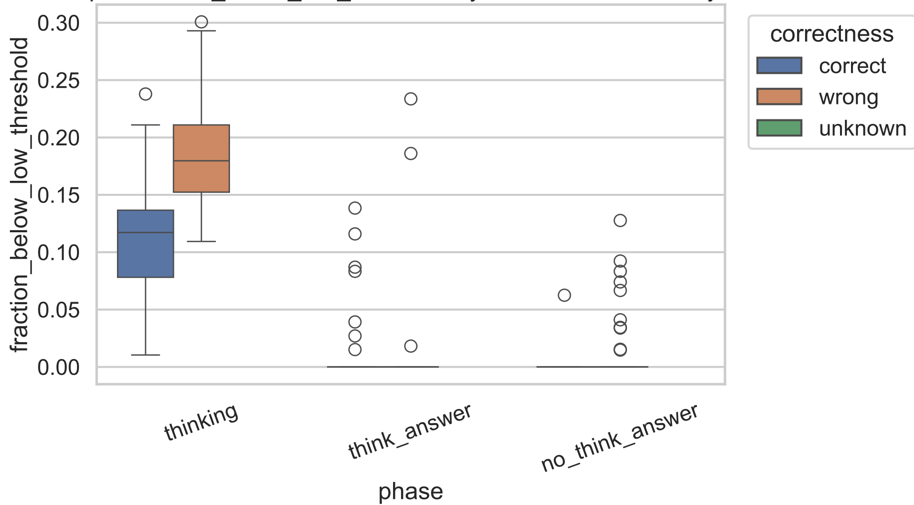
Exp C fraction_below_low_threshold by correctness, 1.7B, layer 6
