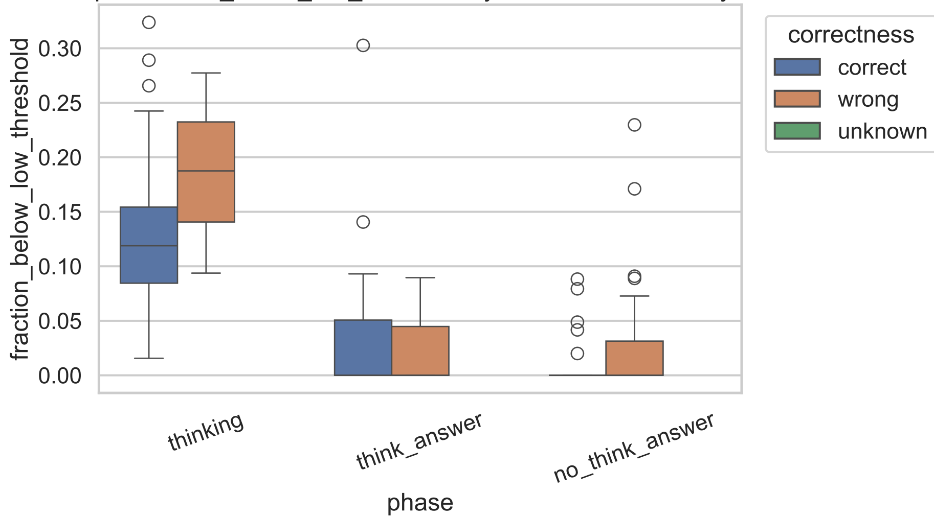
Exp C fraction_below_low_threshold by correctness, 14B, layer 6
