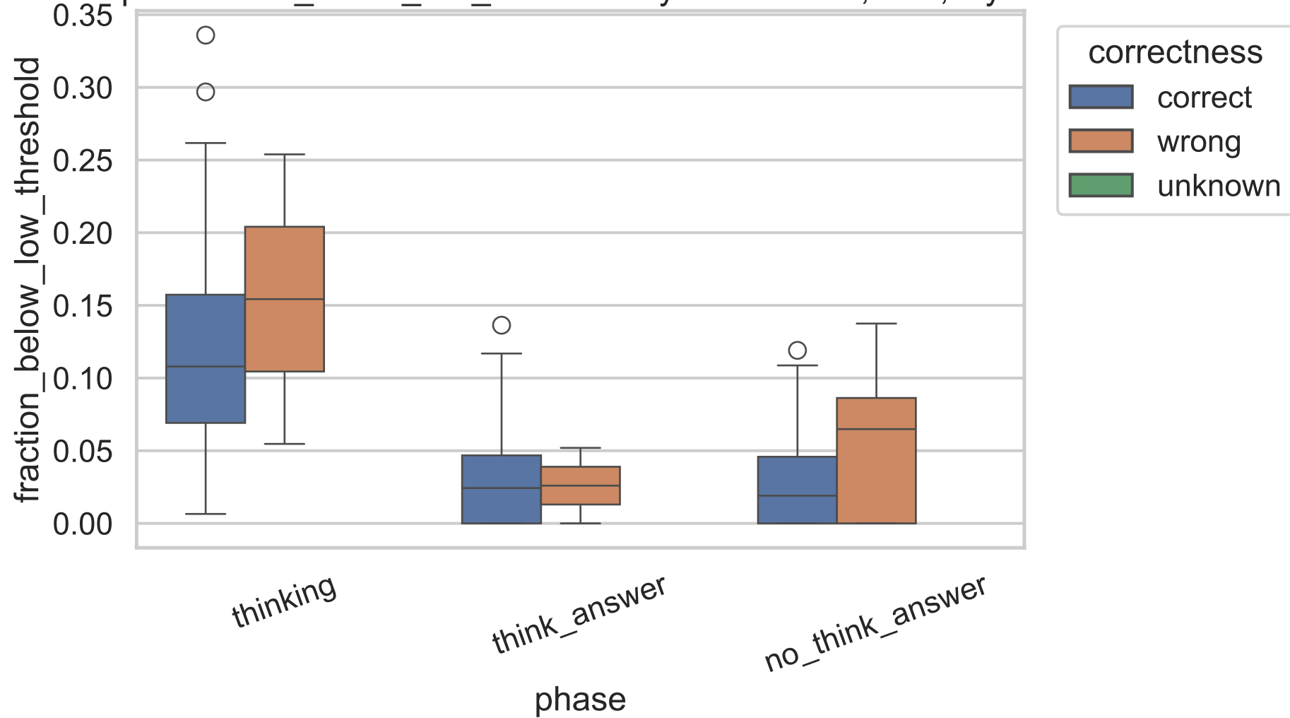
Exp C fraction_below_low_threshold by correctness, 32B, layer 13
