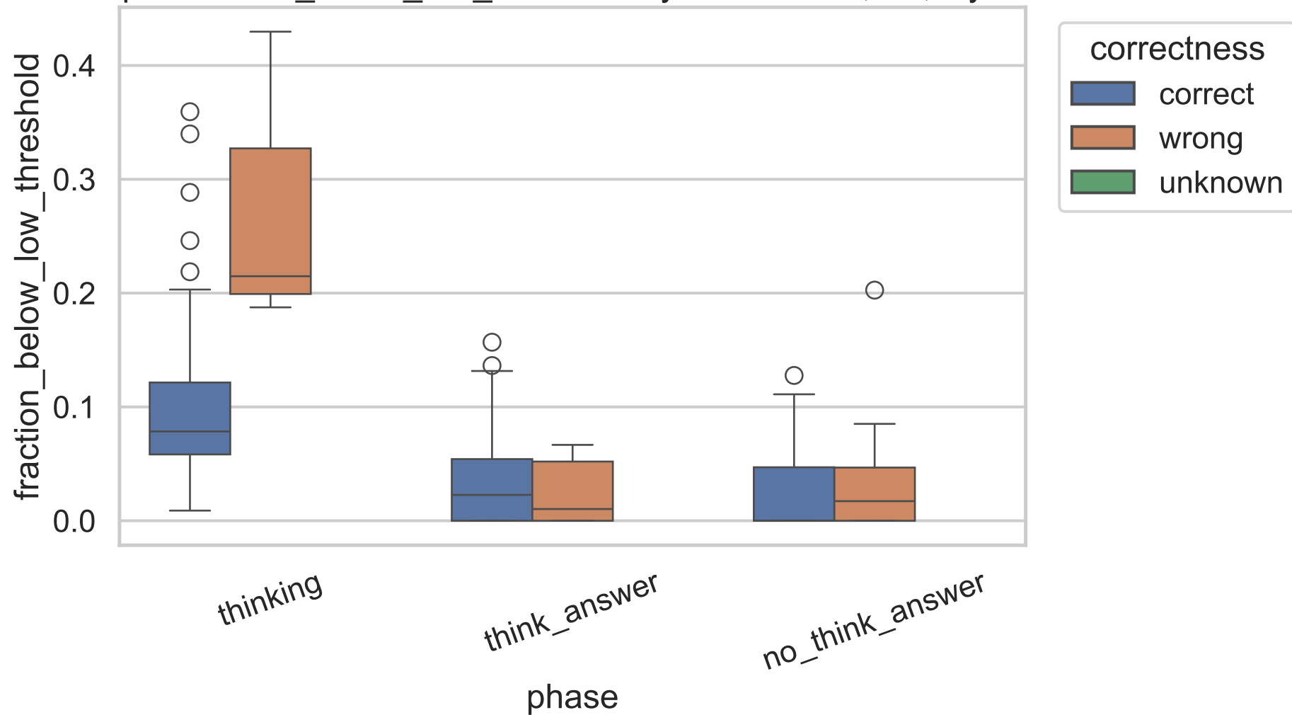
Exp C fraction_below_low_threshold by correctness, 4B, layer 20
