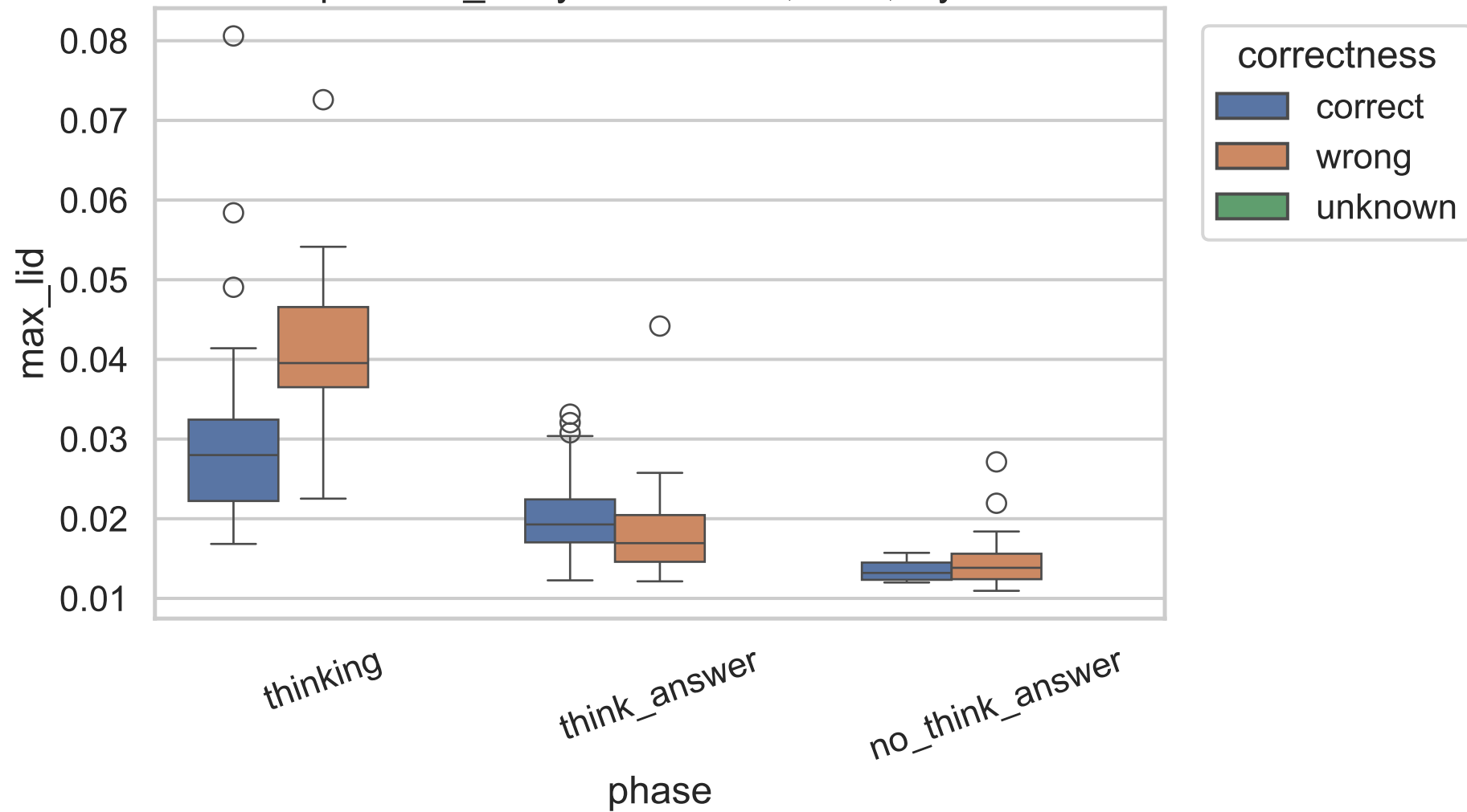
Exp C max_lid by correctness, 1.7B, layer 13
