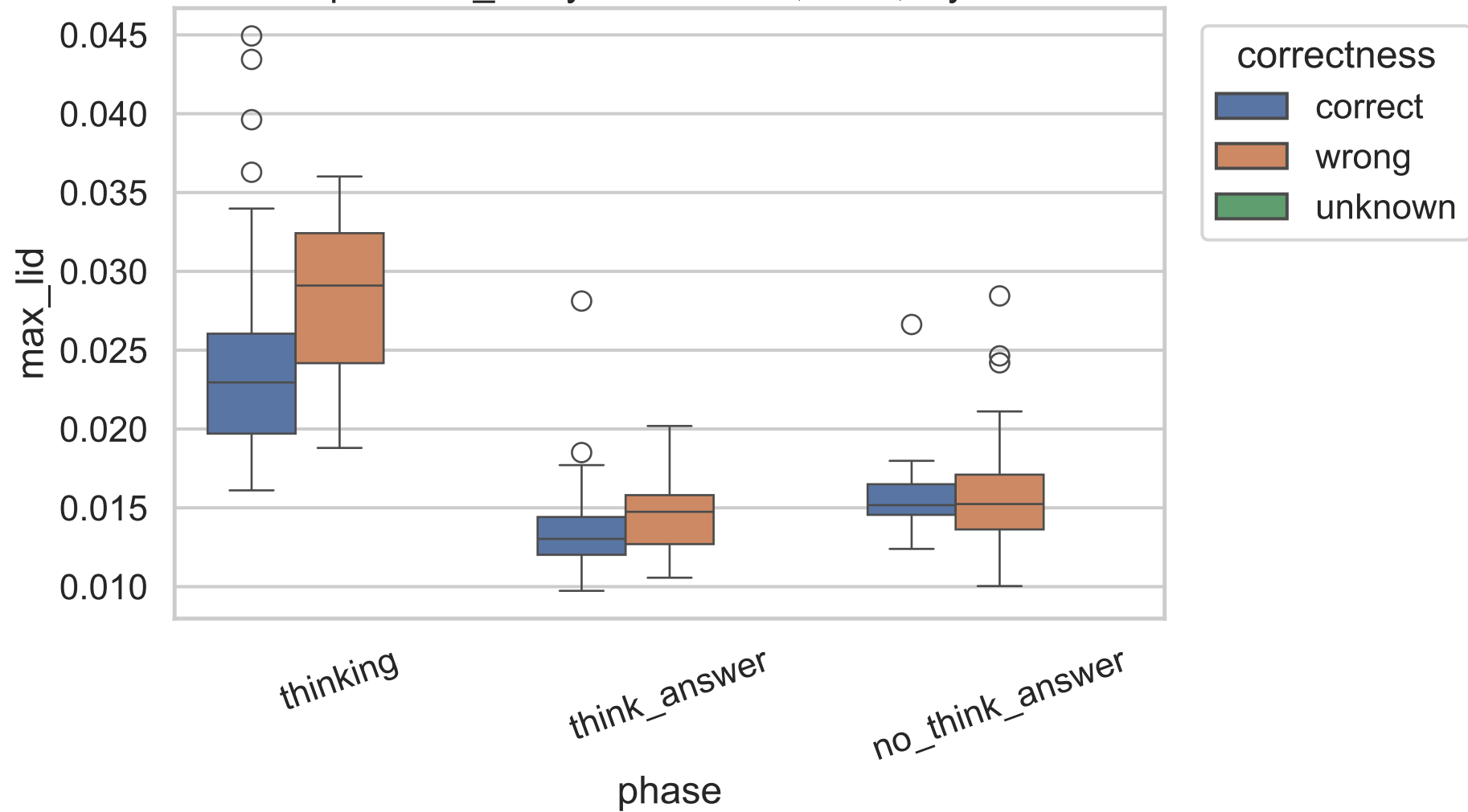
Exp C max_lid by correctness, 1.7B, layer 20
