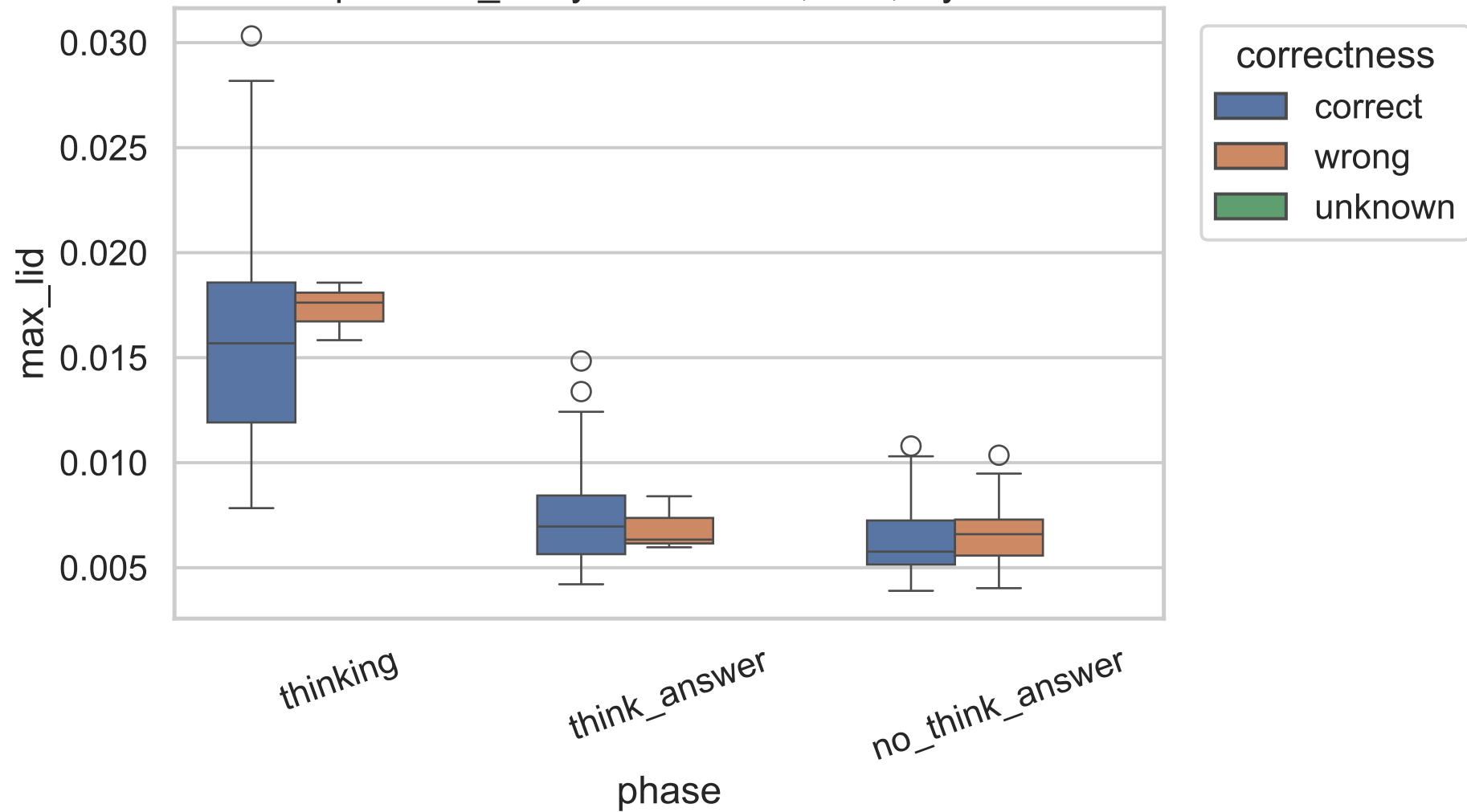
Exp C max_lid by correctness, 14B, layer 13
