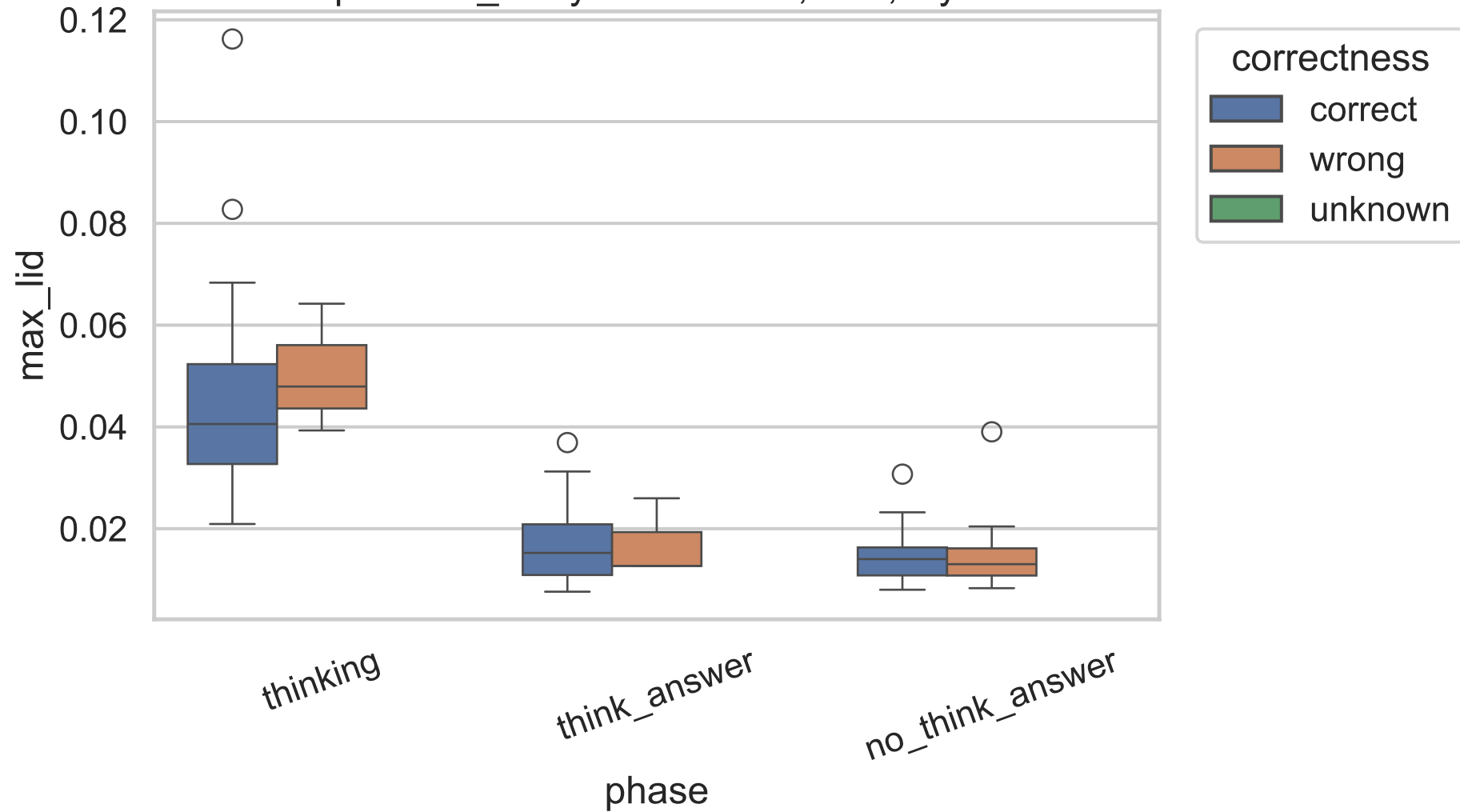
Exp C max_lid by correctness, 14B, layer 6
