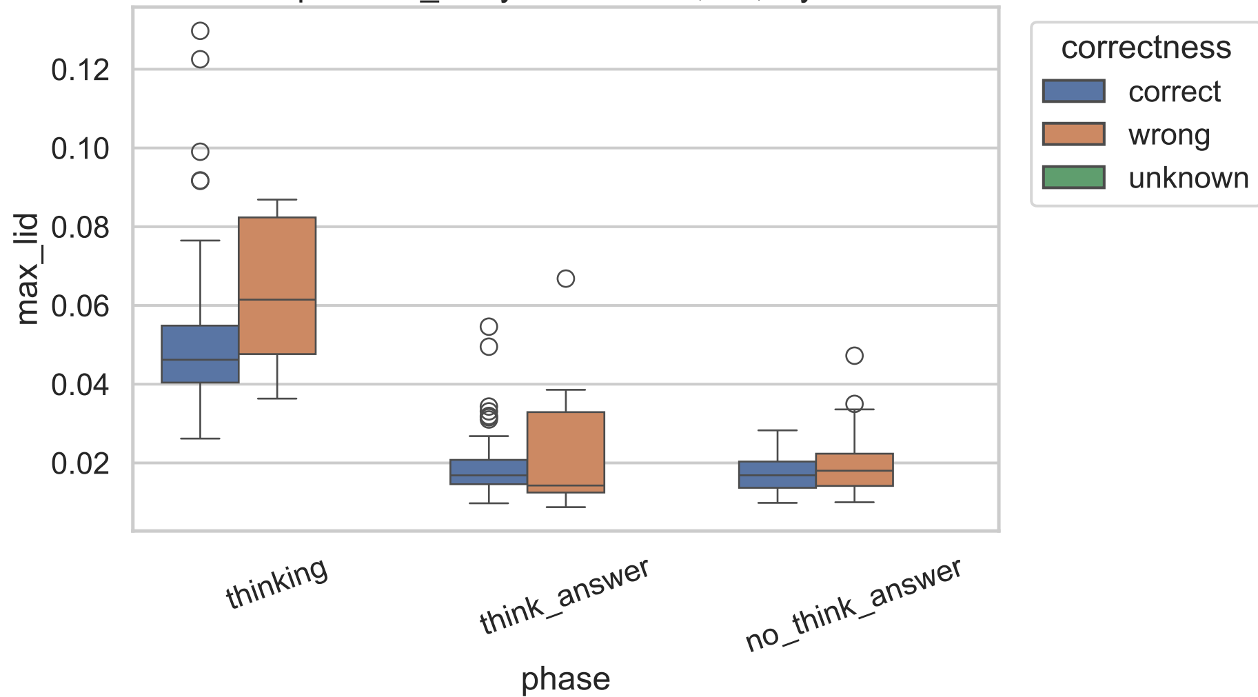
Exp C max_lid by correctness, 4B, layer 6
