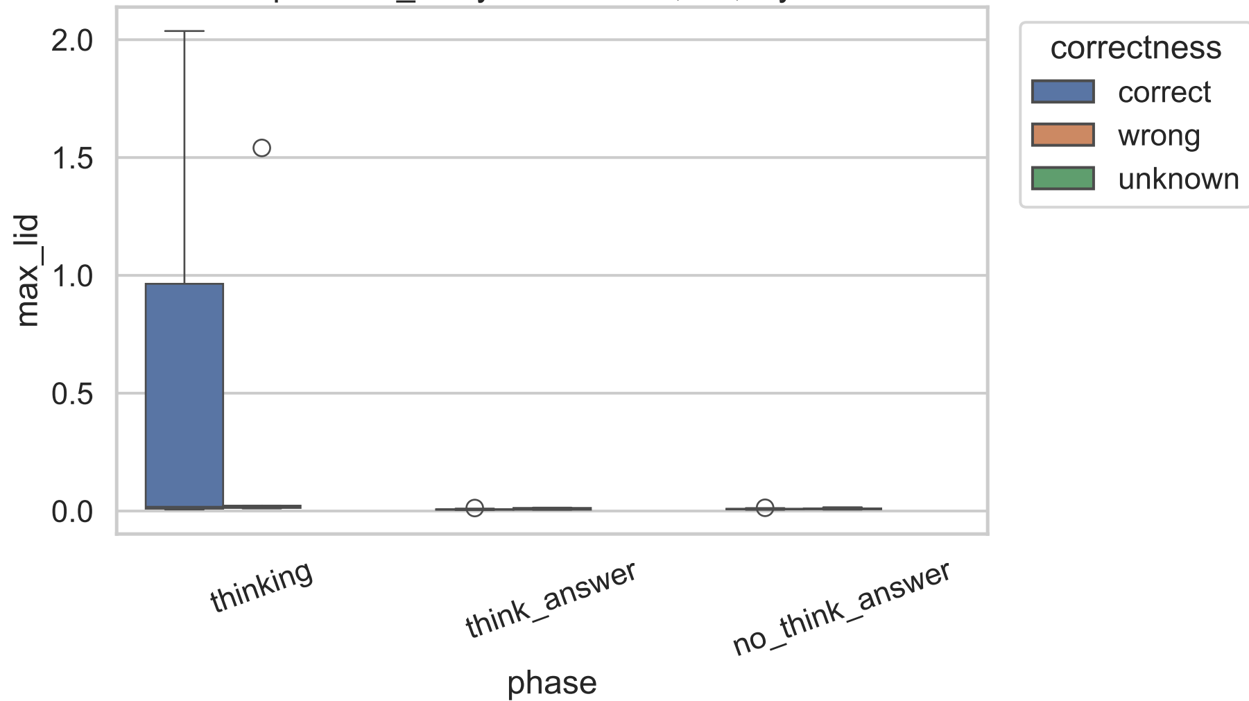
Exp C max_lid by correctness, 8B, layer 20
