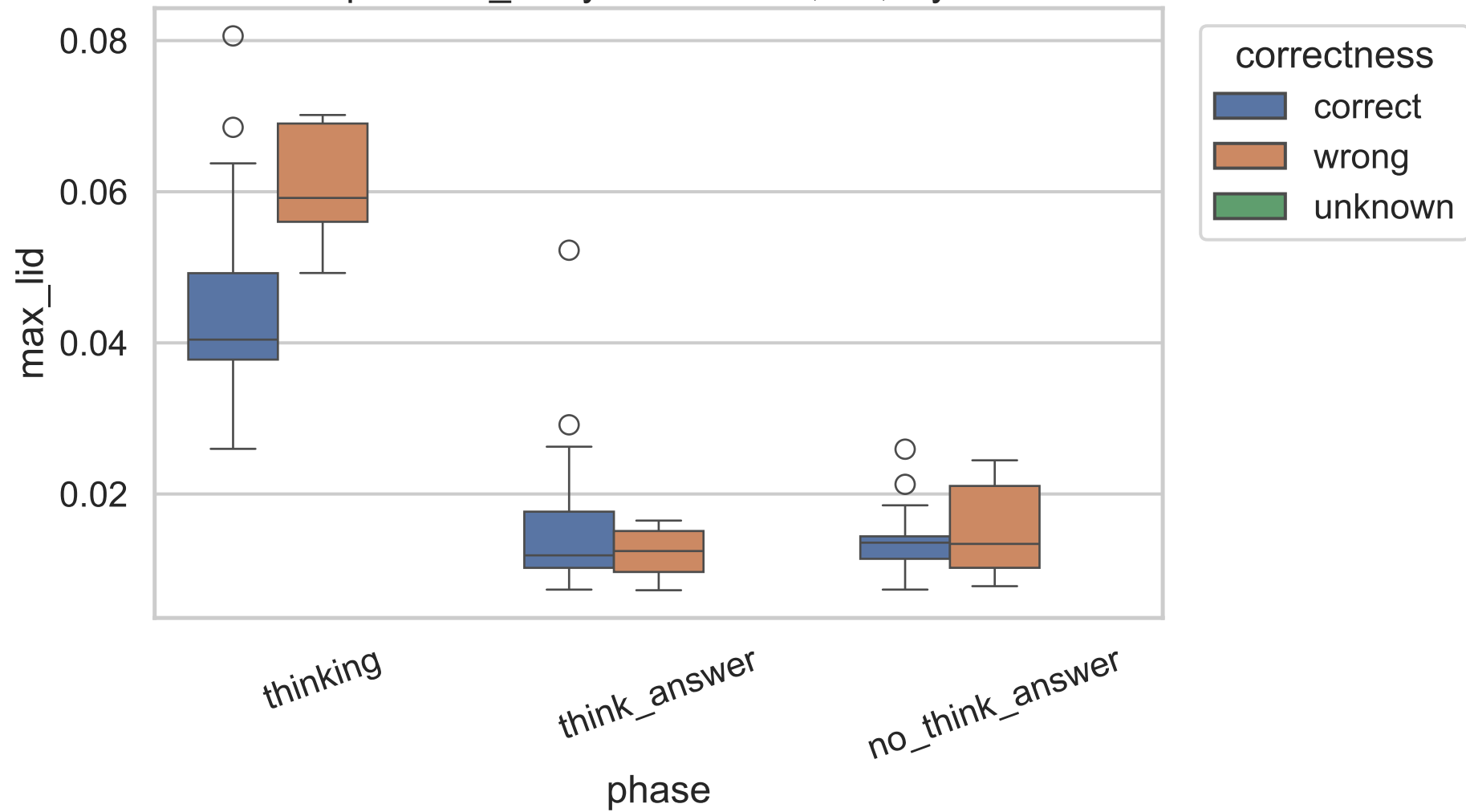
Exp C max_lid by correctness, 8B, layer 6
