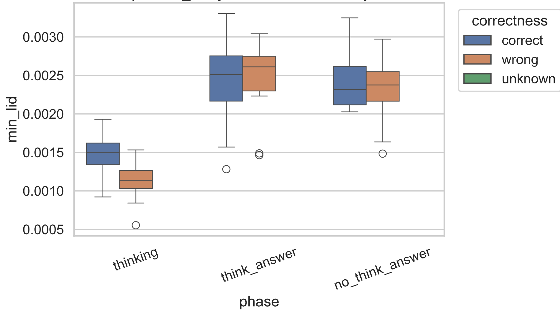
Exp C min_lid by correctness, 1.7B, layer 13
