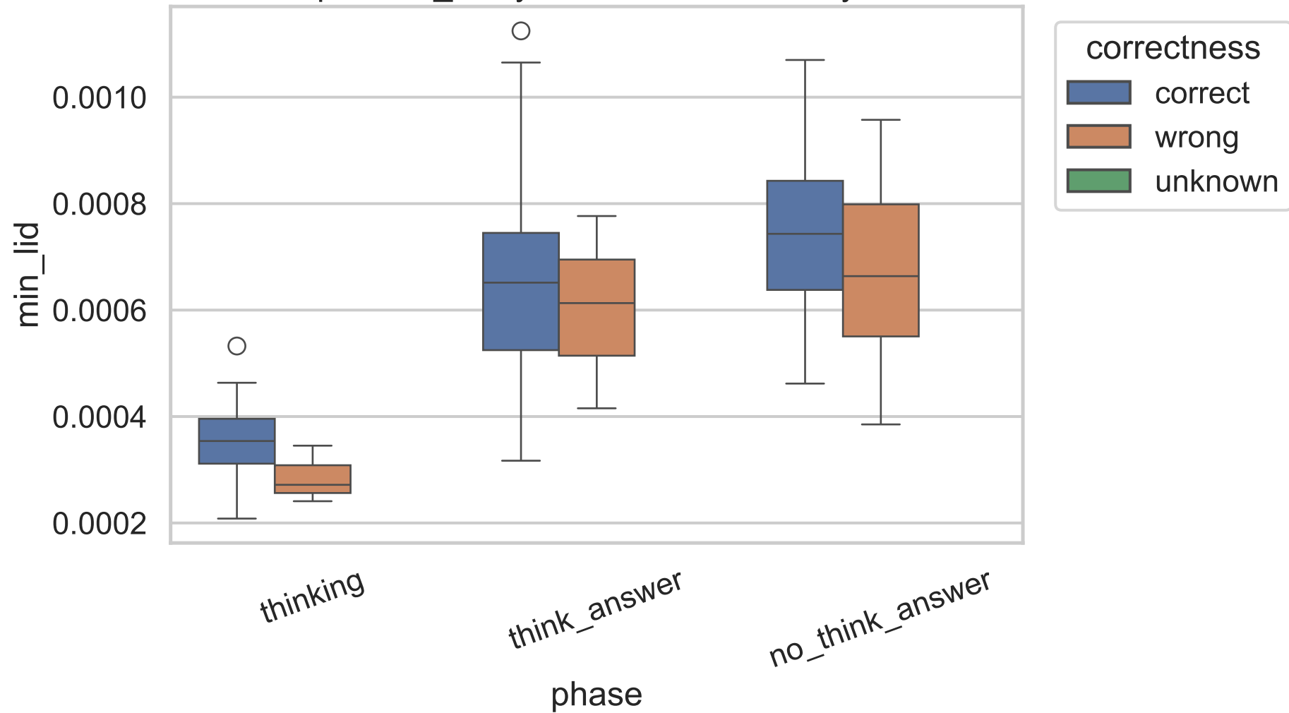
Exp C min_lid by correctness, 14B, layer 6
